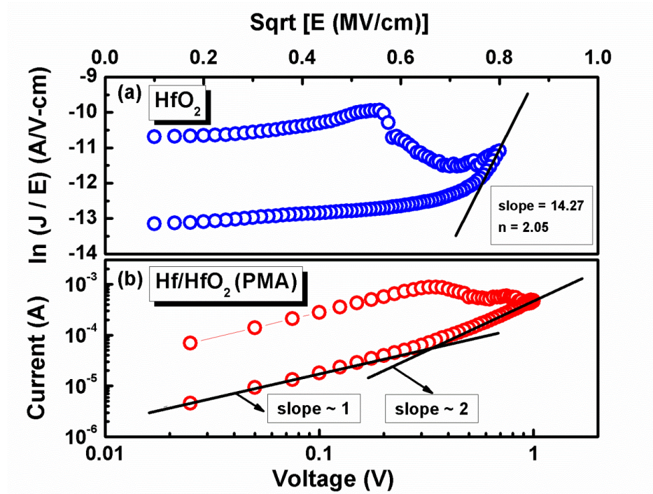
Figure 2. Curve fitting in Pt/HfO 2 /TiN devices (a) Poole-Frenkel emission and in Pt/Hf/HfO 2 /TiN devices (b) SCLC mechanism.
